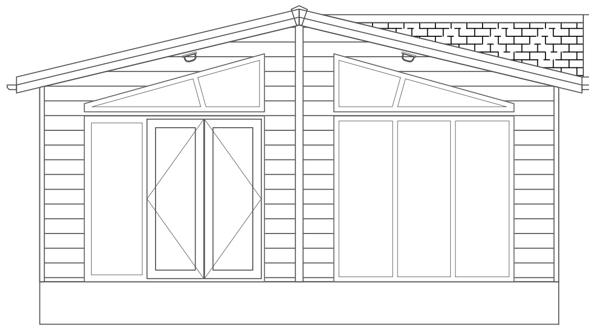
Elevation C
