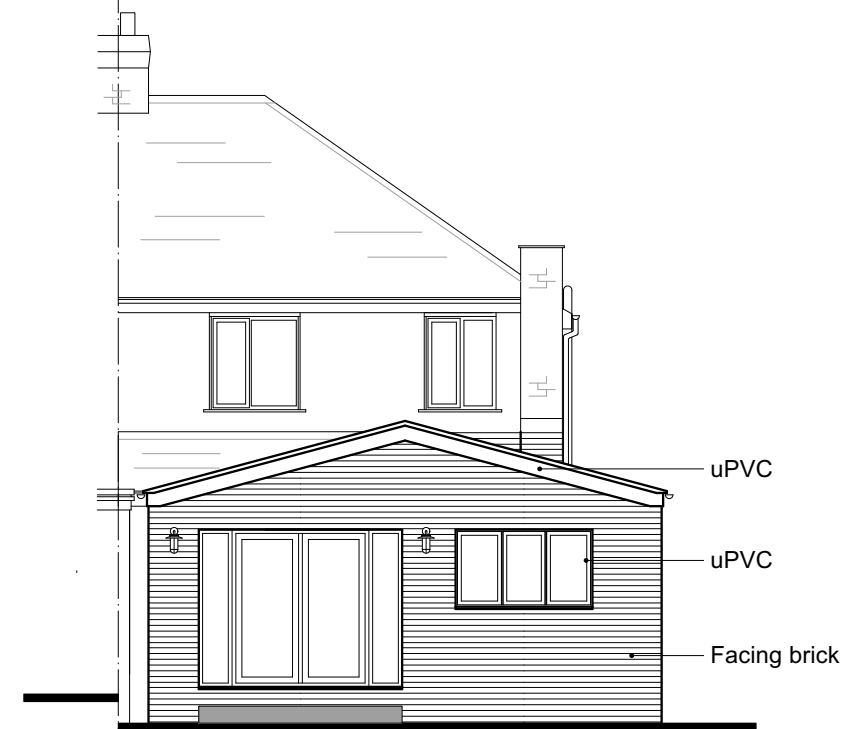
Proposed Rear Elevation View 'C' 1:100
