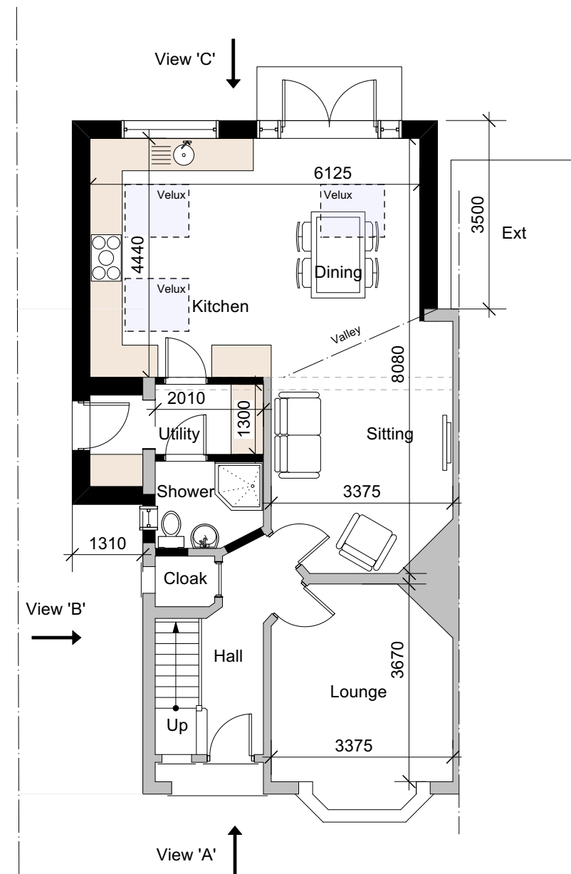
Proposed Ground Floor Plan 1:50
