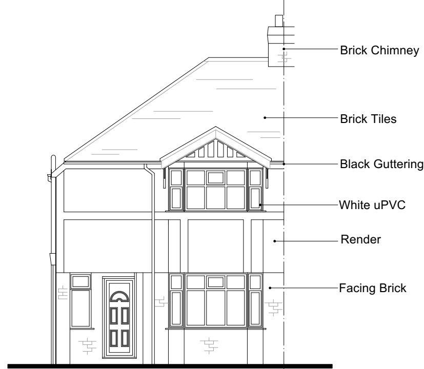
Existing Front Elevation View 'A' 1:100
