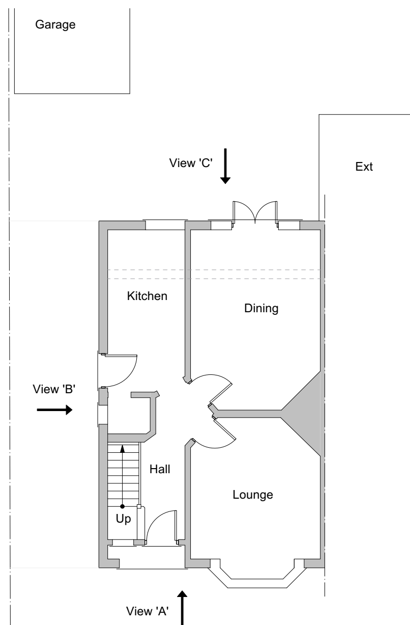
Existing Ground Floor Plan 1:50
