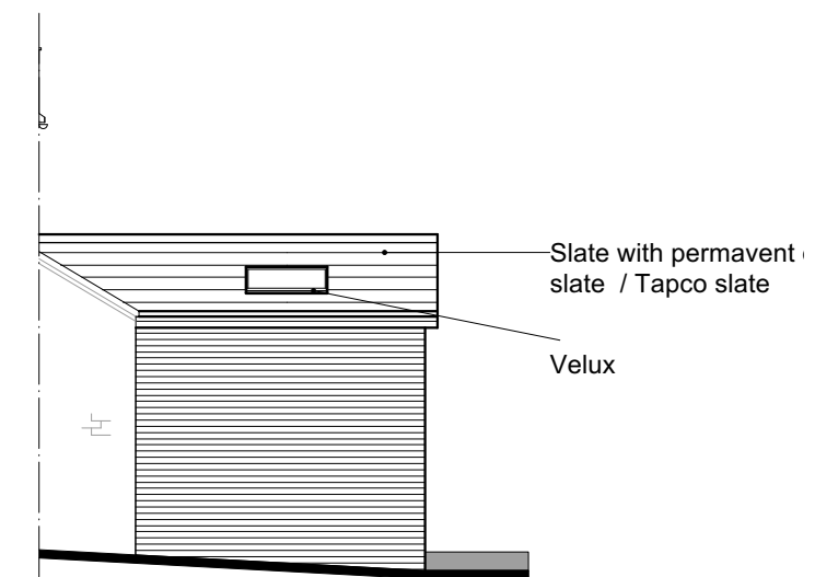
Proposed Side Elevation View 'D' 1:100
