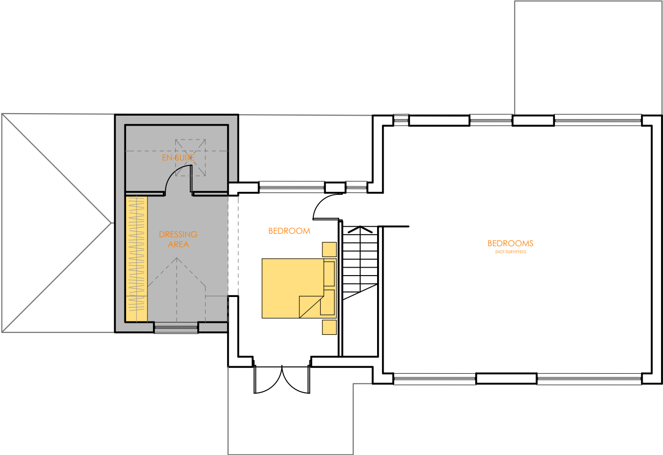
2 FIRST FLOOR PLAN
