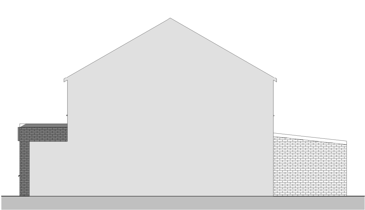
Side Elevation 1 : 100
