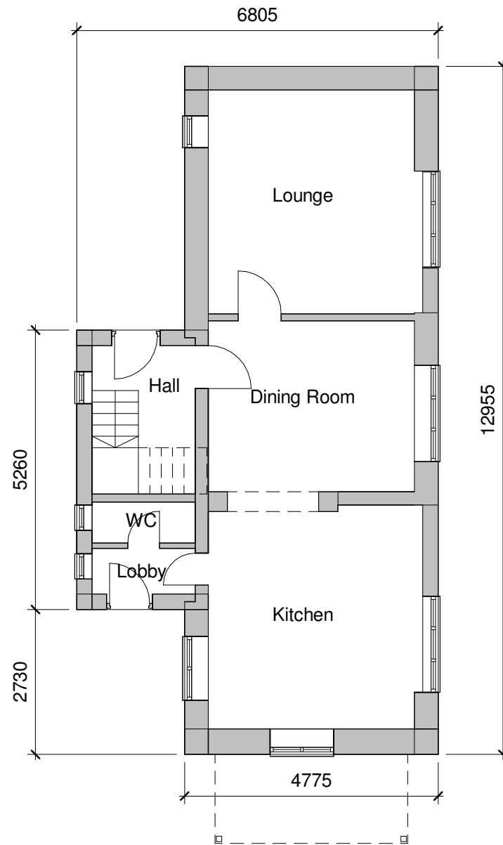
Ground Floor 1 : 100
