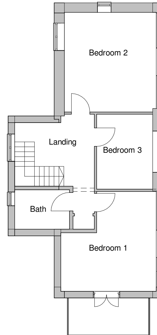
First Floor 1 : 100
