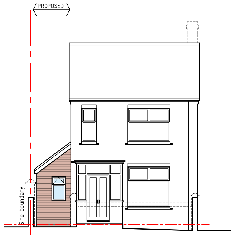
Front Elevation 1:100
