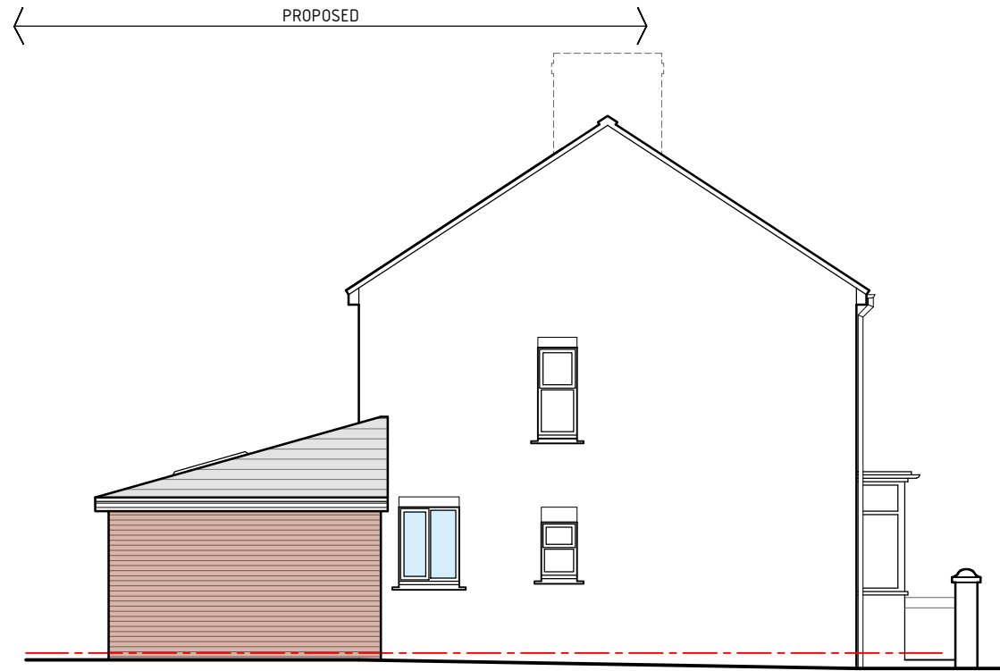
Side-01 Elevation 1:100
