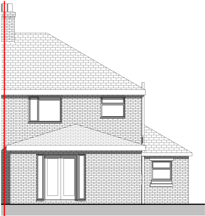
Rear Elevation 1 : 100
