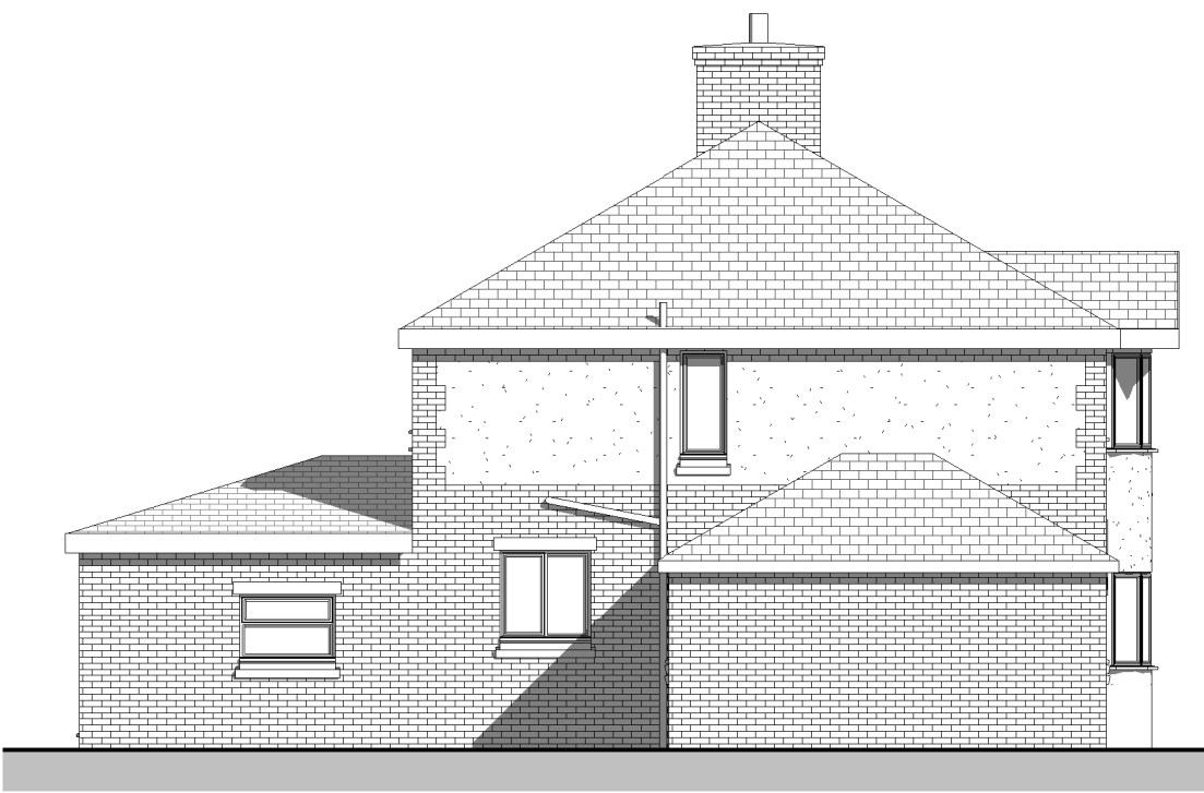
Side Elevation 1 : 100
