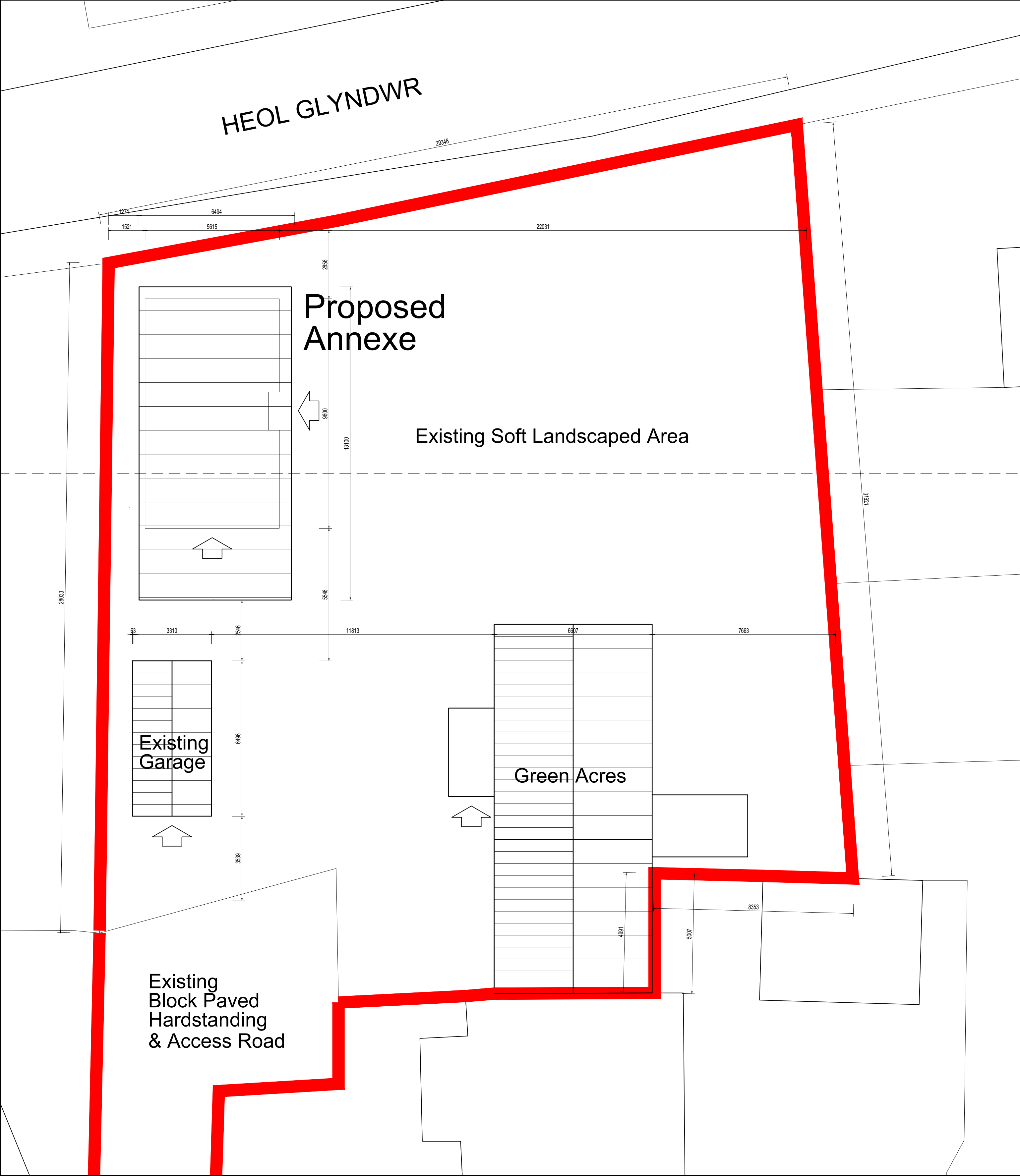
Proposed Site Layout (1:100)
