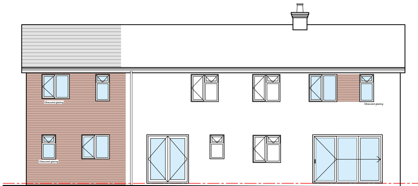
Rear Elevation
