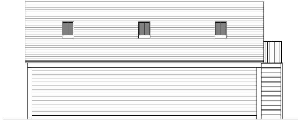
REAR ELEVATION
