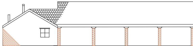
West Elevation
