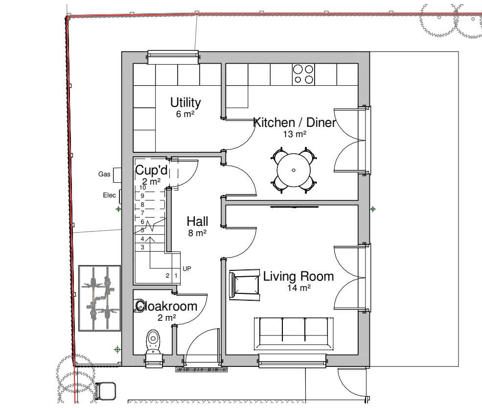
3 Ground Floor Plan 1 : 100
