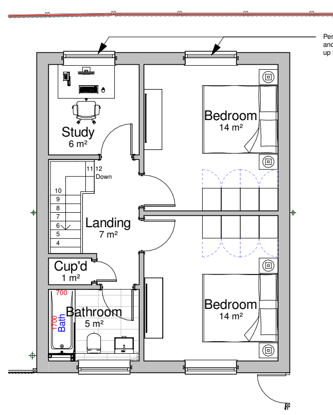
4 First Floor Plan 1 : 100
