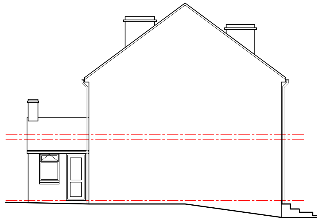
1 Coed Richard - Side elevation
