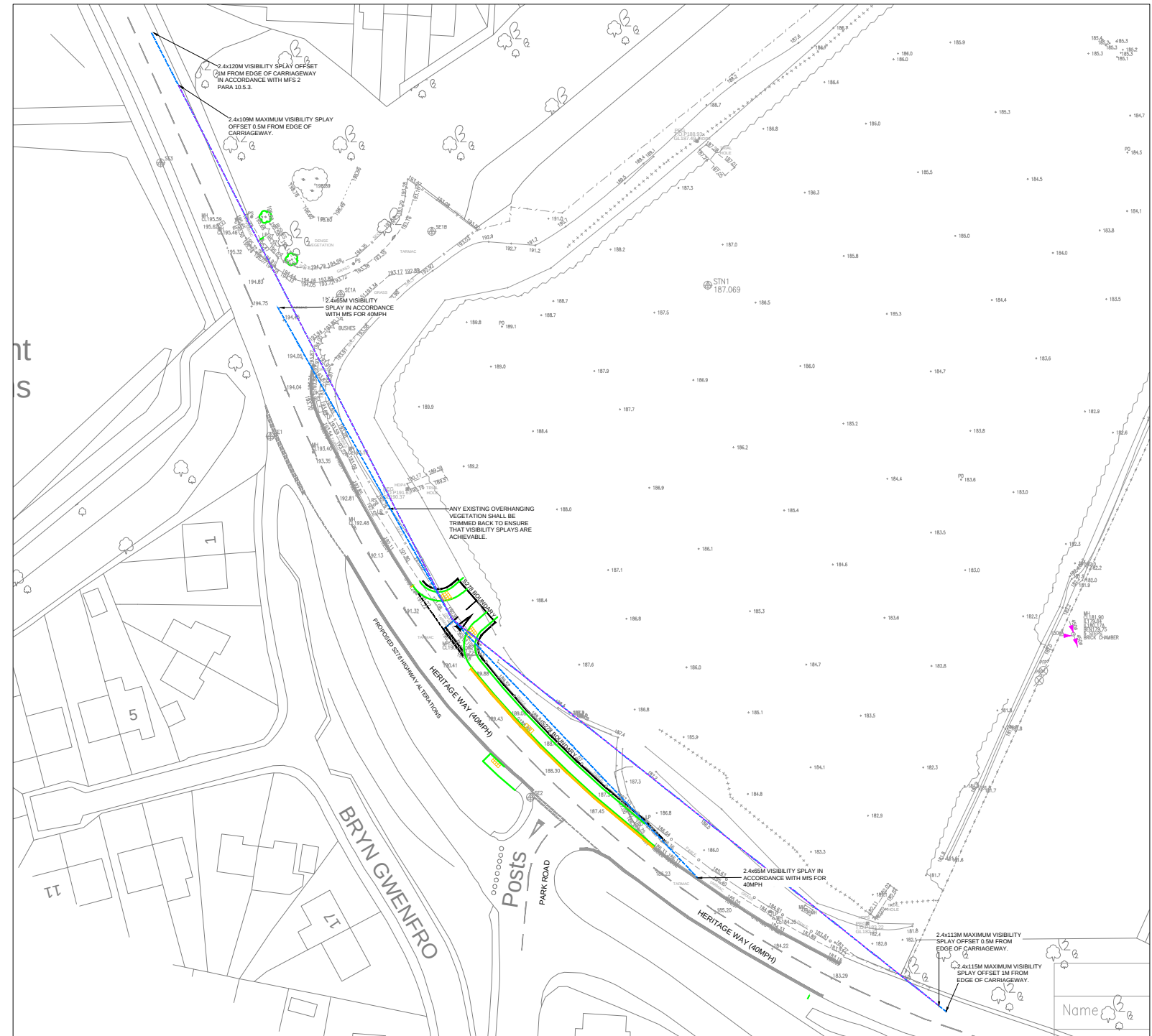
VISIBILITY SPLAYS @ 1:1000 SCALE
