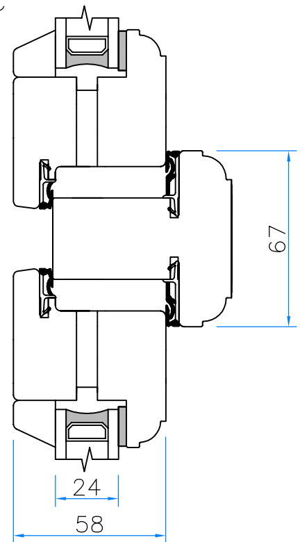
SECTION C-C
