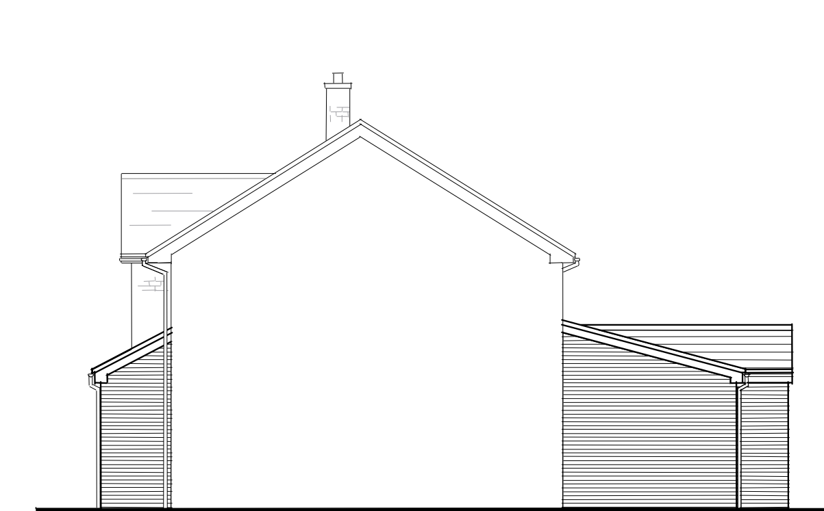
Proposed Side Elevation View D - 1:100
