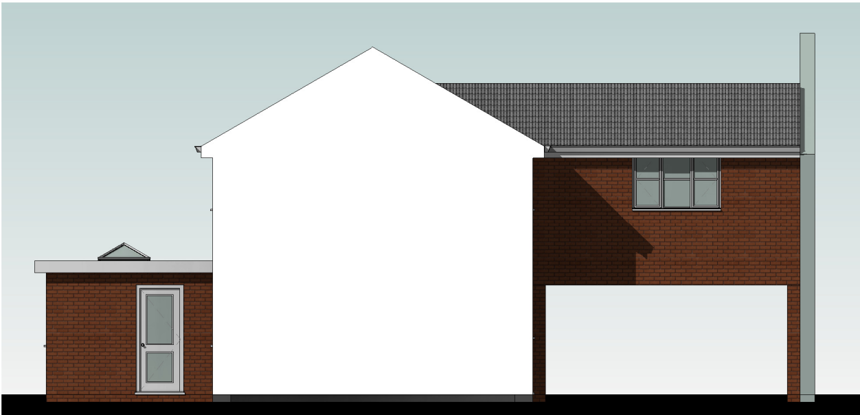
West Elevation 1 : 100
