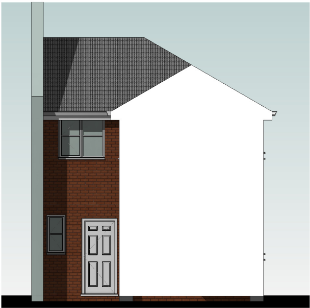
South Elevation 1 : 100
