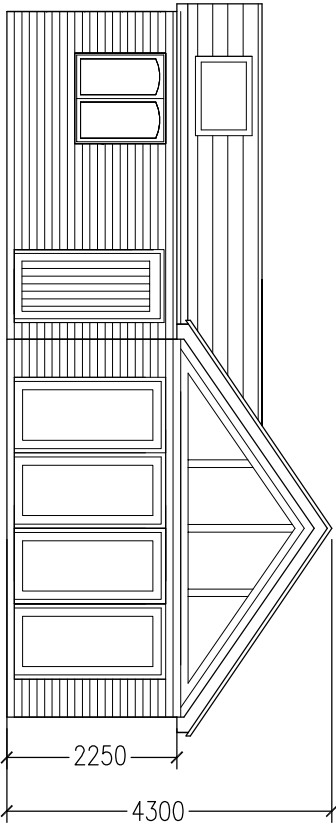
WEST ELEVATION CANALSIDE
