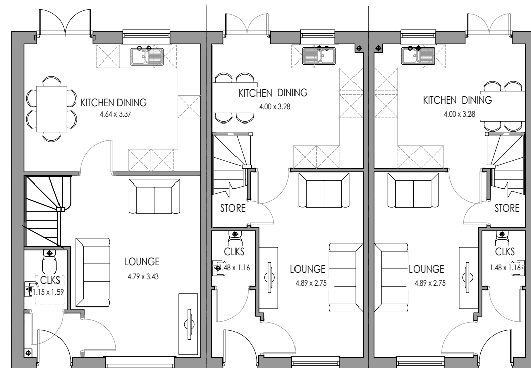
ELWY OPP GROUND FLOOR
