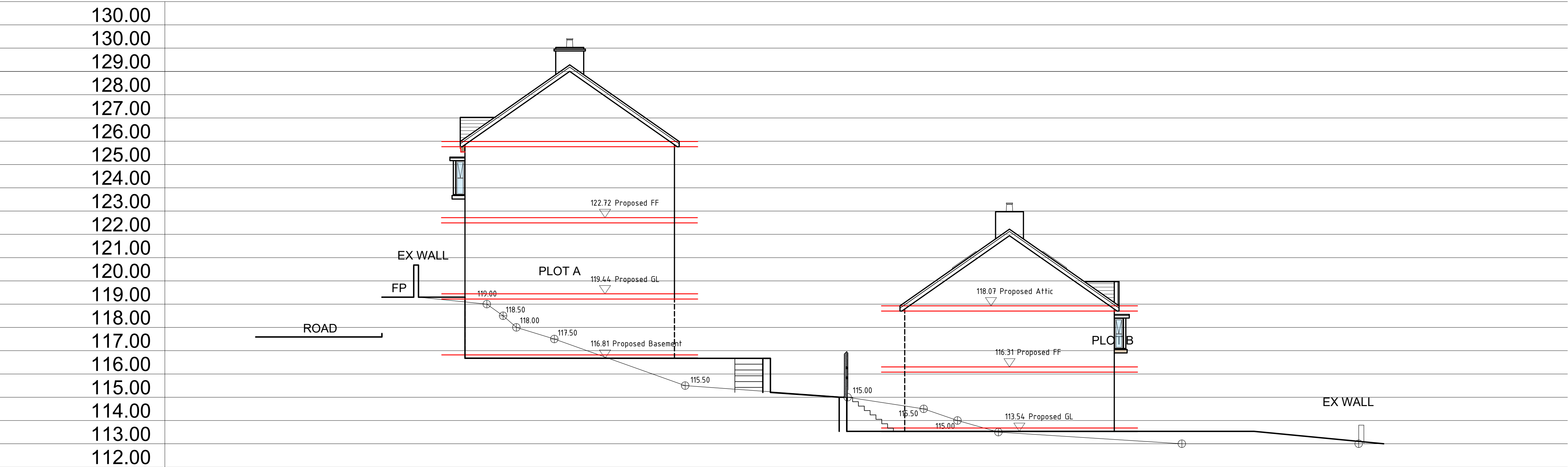
Section A-A as Proposed
