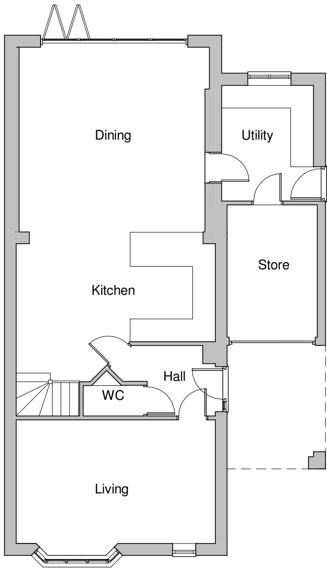
Ground Floor 1 : 100
