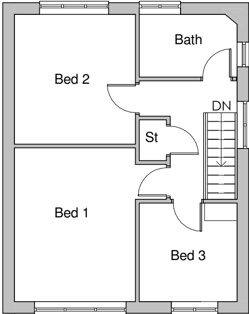
First Floor 1 : 100
