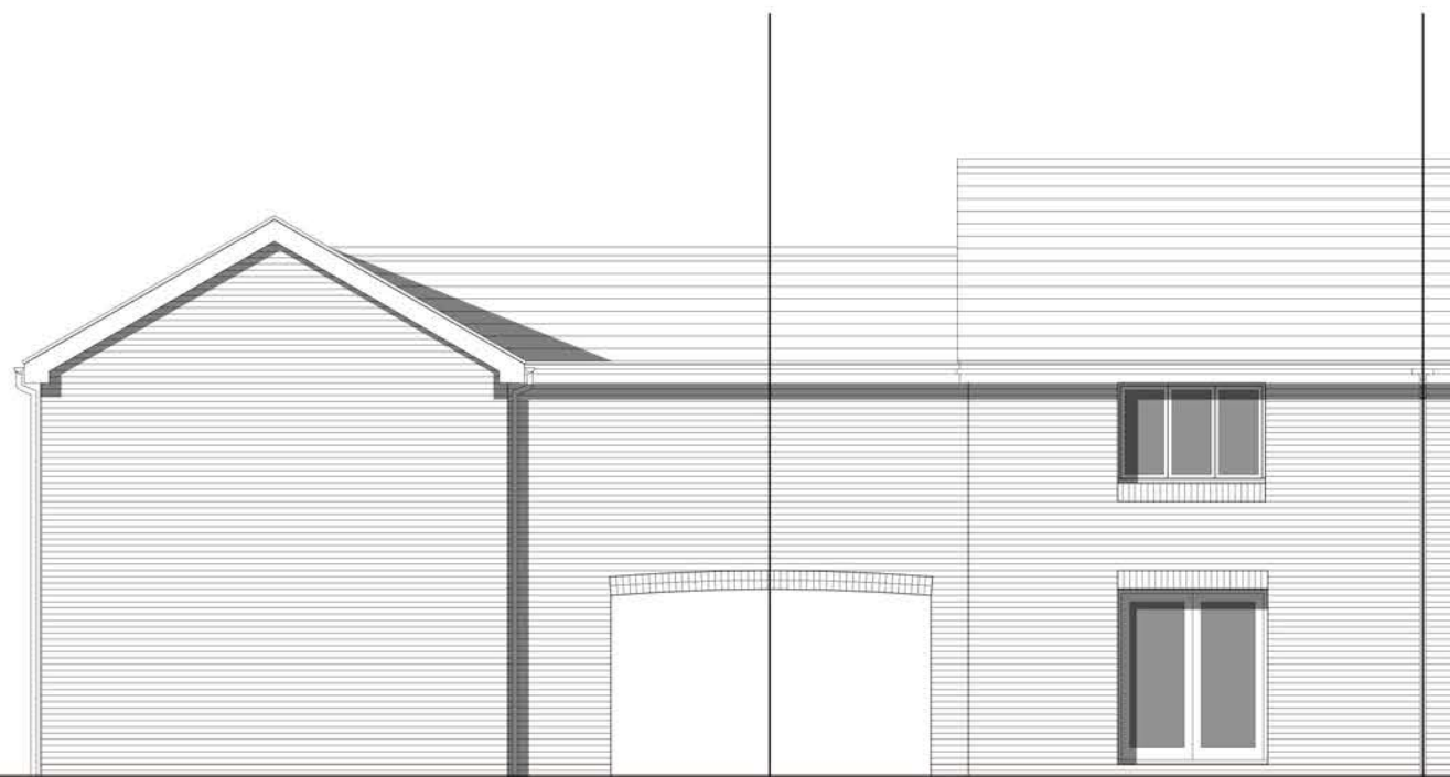
Rear Elevation
