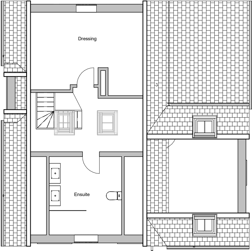
Level 3 - Second Floor 1 : 100
