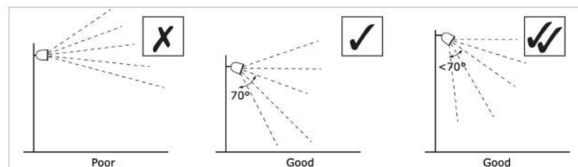
Figure 3 Luminaire aiming angles
