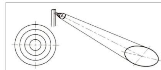
Type A: Floodlight/projector producing a symmetrical beam
