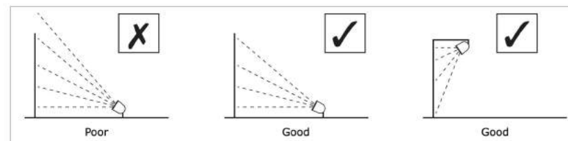
Figure 4 Façade illumination
