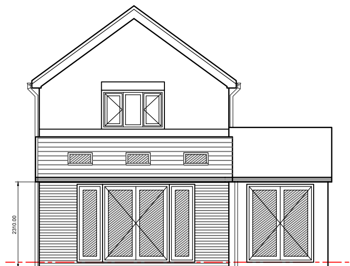
Rear Elevation
