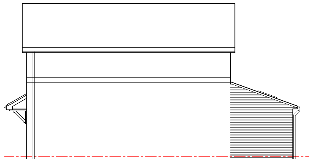
Side 01 Elevation
