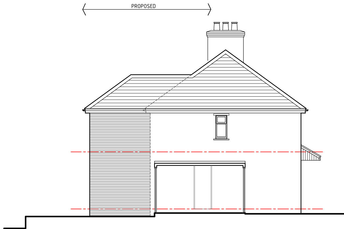
Side-01 elevation 1:100
