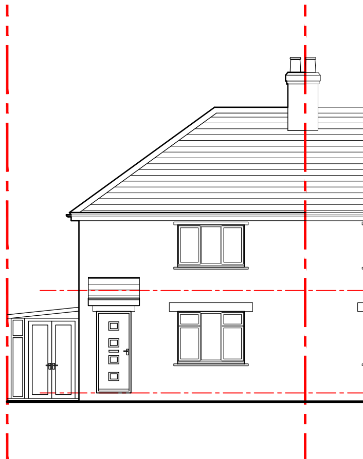
Front elevation 1:100
