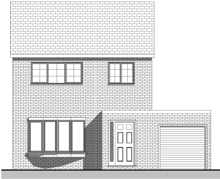
Front Elevation 1 : 100
