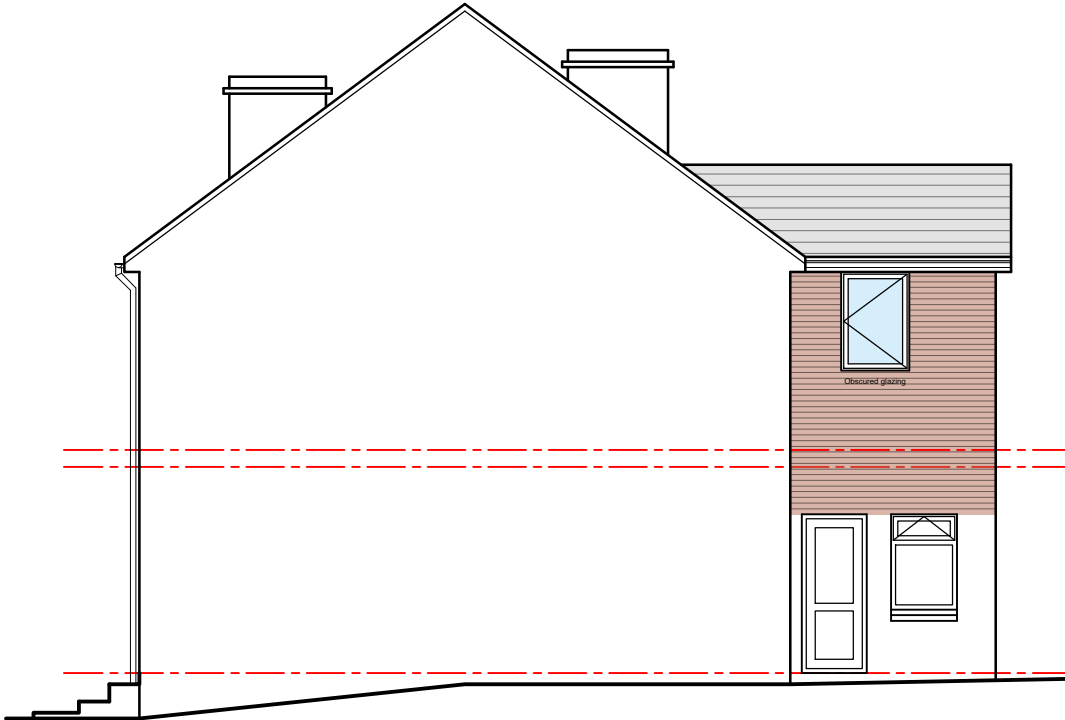
2 Coed Richard - Side elevation
