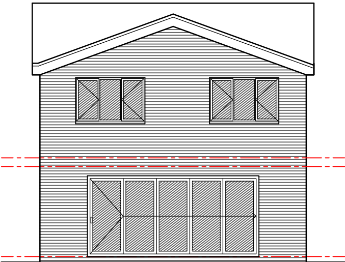
Rear Elevation
