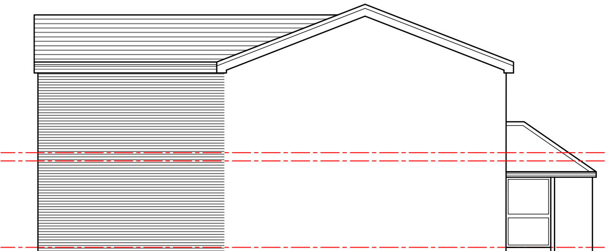
Side Elevation-02
