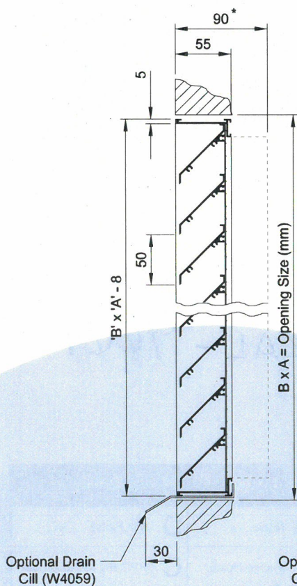
W4050 Recessed Frame
