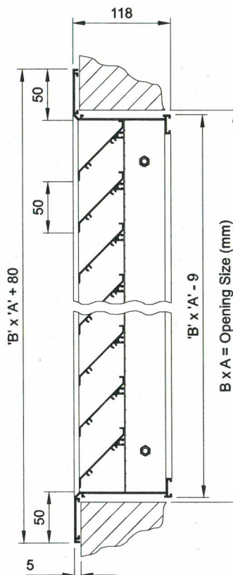
W5250 Flanged Frame: Multi-Panel with continuous blade appearance
