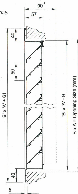
W5050 Flanged Frame
