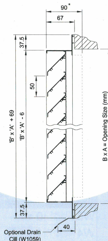
W1050 Reversed Angle Frame
