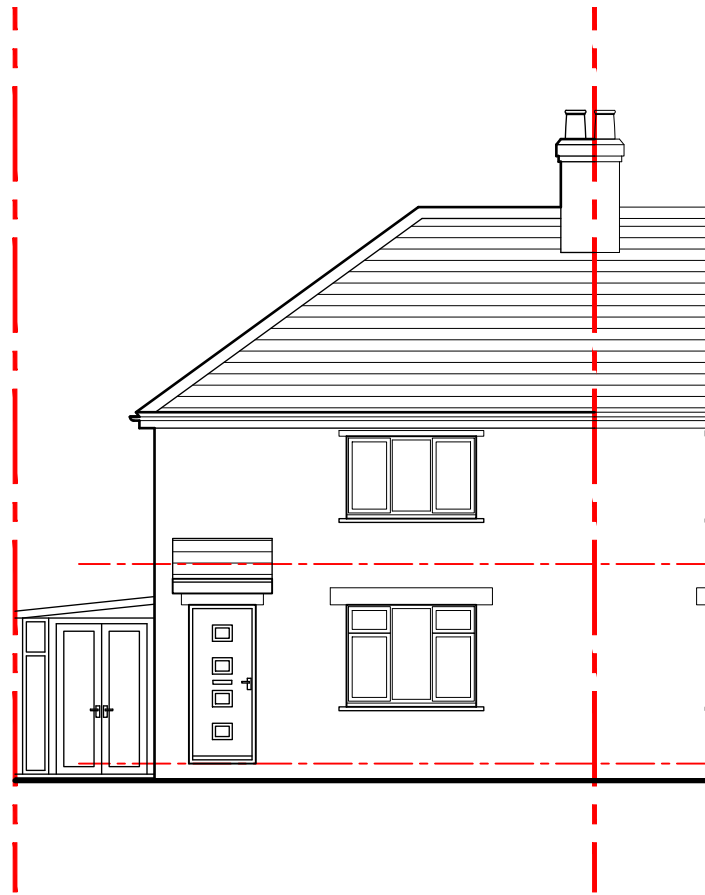
Front elevation 1:100
