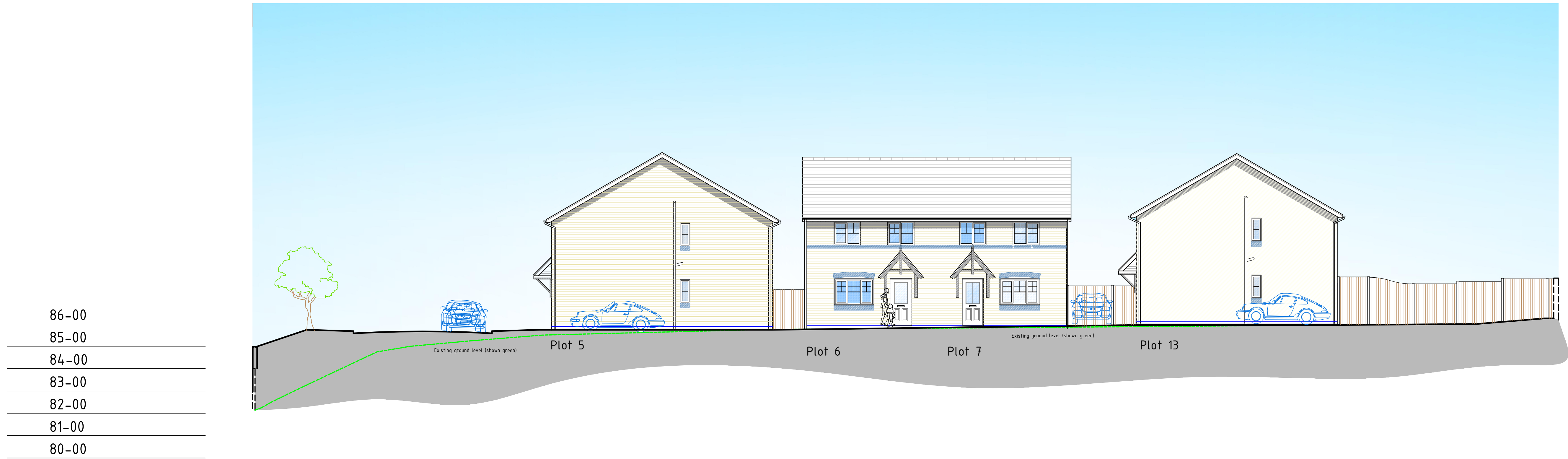
Section B-B as Proposed
