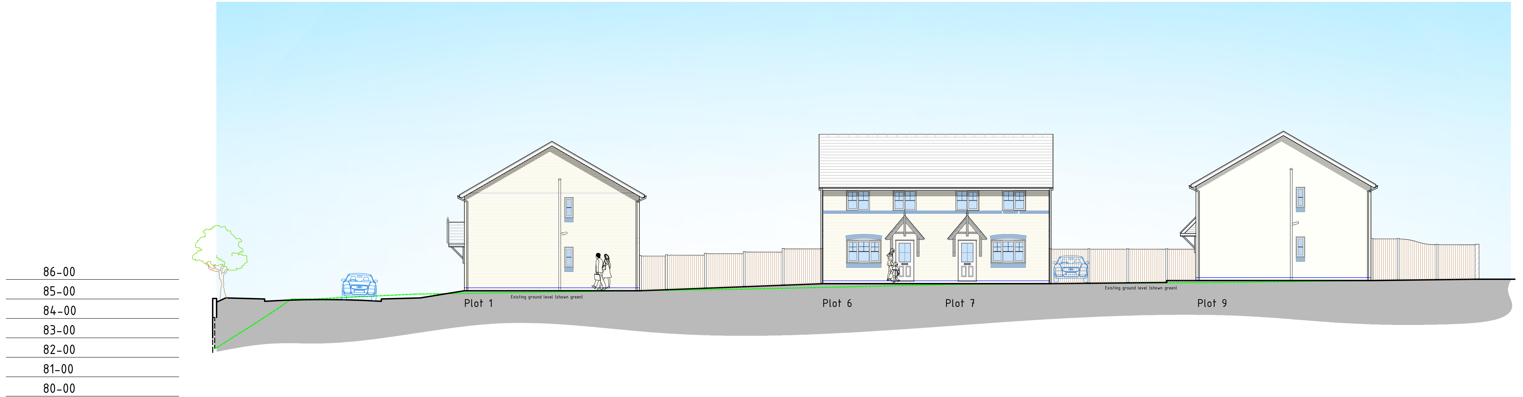
Section A-A as Proposed
