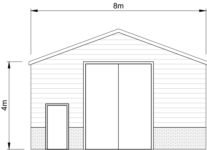
East Elevation
