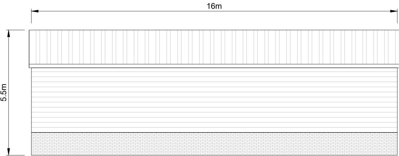
North Elevation
