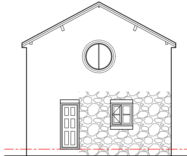
Side 01 Elevation
