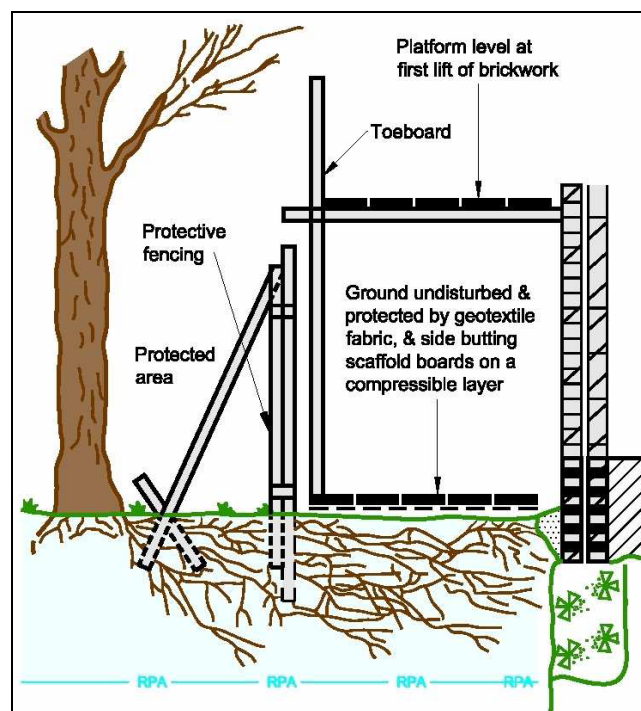
Plate 1- protective boards & scaffolding to be installed
