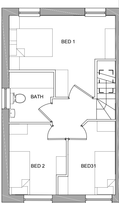
First Floor Plan [1:100] Floor Area Approx 36m 2
