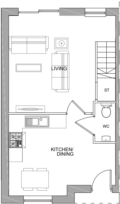
Ground Floor Plan [1:100] Floor Area Approx 36m 2
