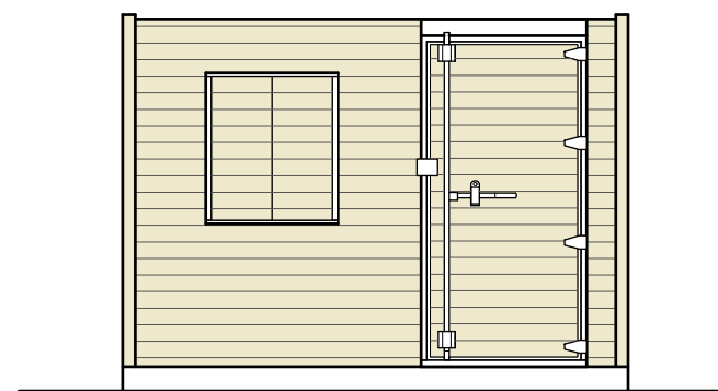
Front Elevation 1:50
