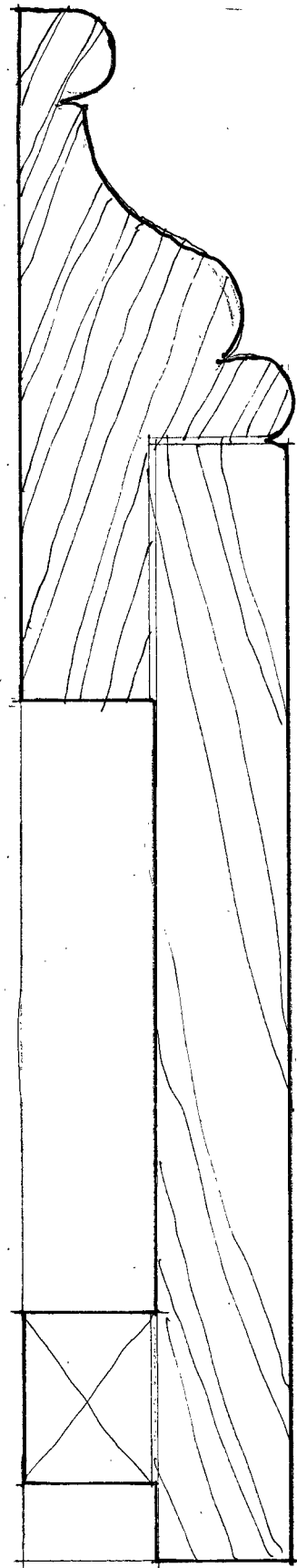
ATTIC SKIRTING
