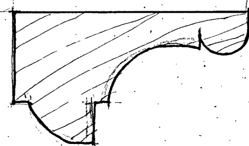
ATTIC ARCHITRAVE
