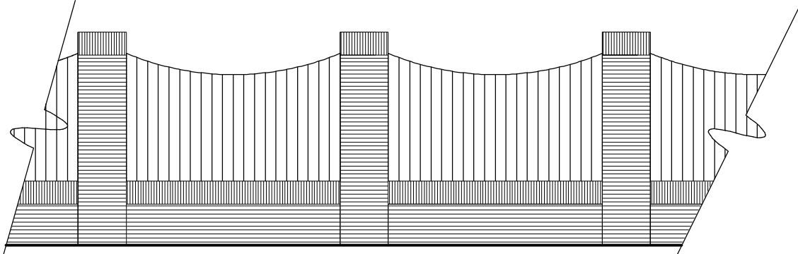
Wall Detail Elevation 1:50 (Rear of dwellings) Indicated on Site Plan as Blue Walls
