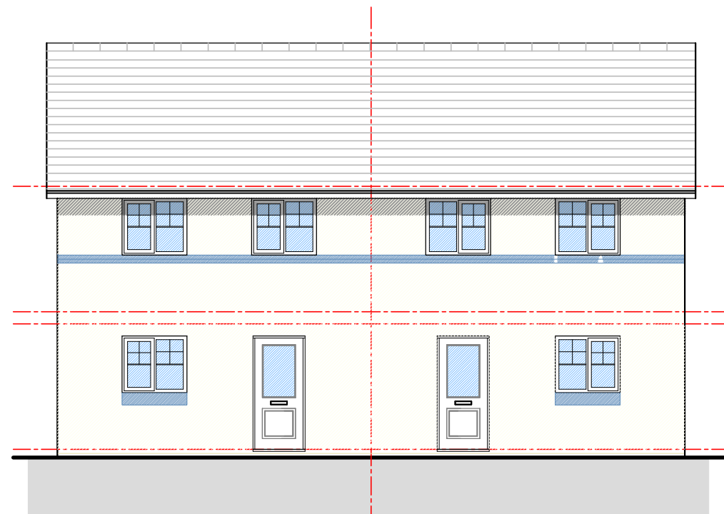
Rear Elevation
