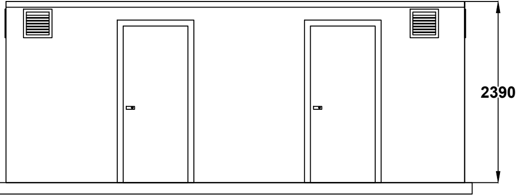
FRONT VIEW
