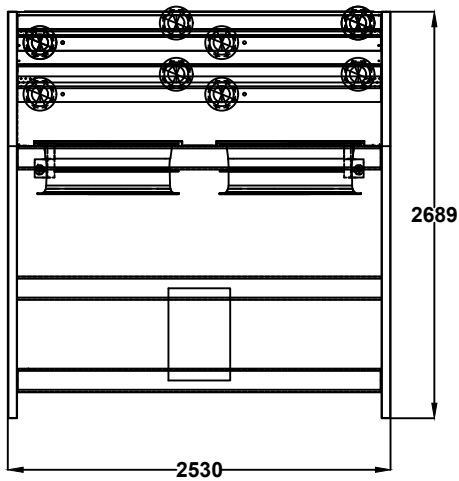
FRONT/REAR VIEW
