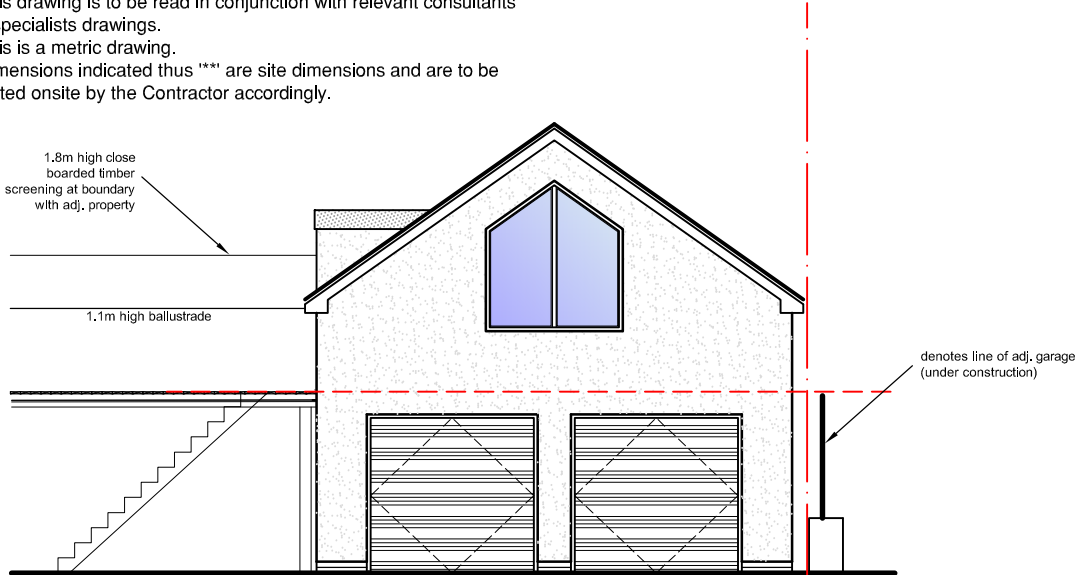
FRONT ELEVATION
