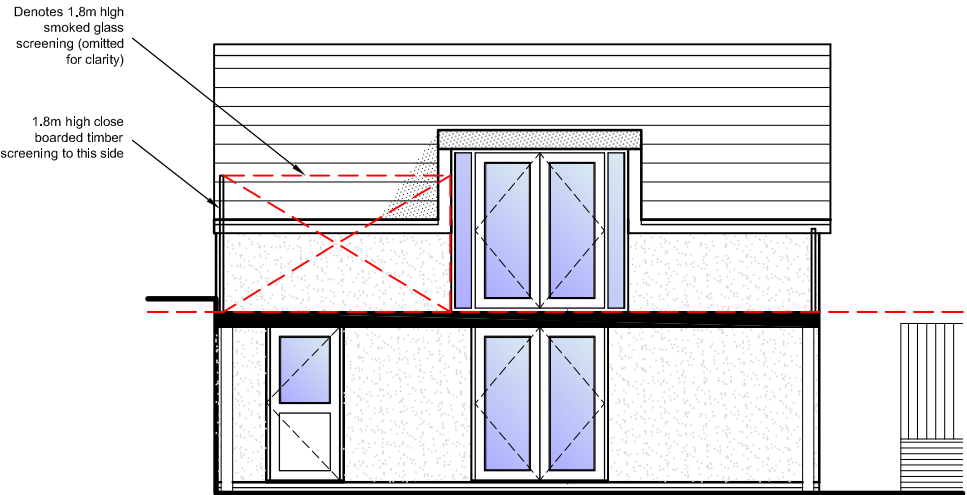
SIDE ELEVATION (part section thru terrace)
