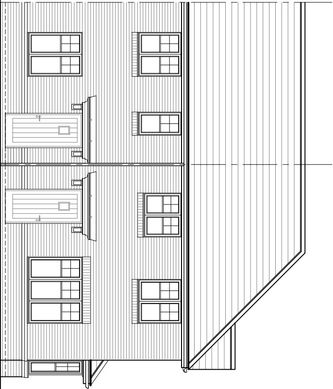
STRATFORD FRONT ELEVATION
