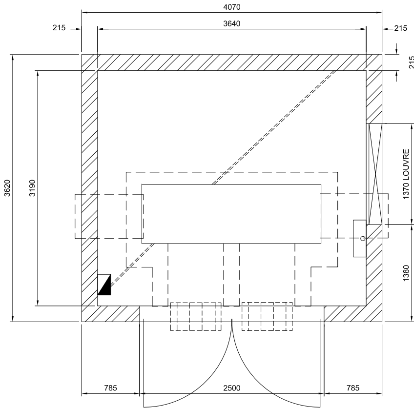
FLOOR PLAN
