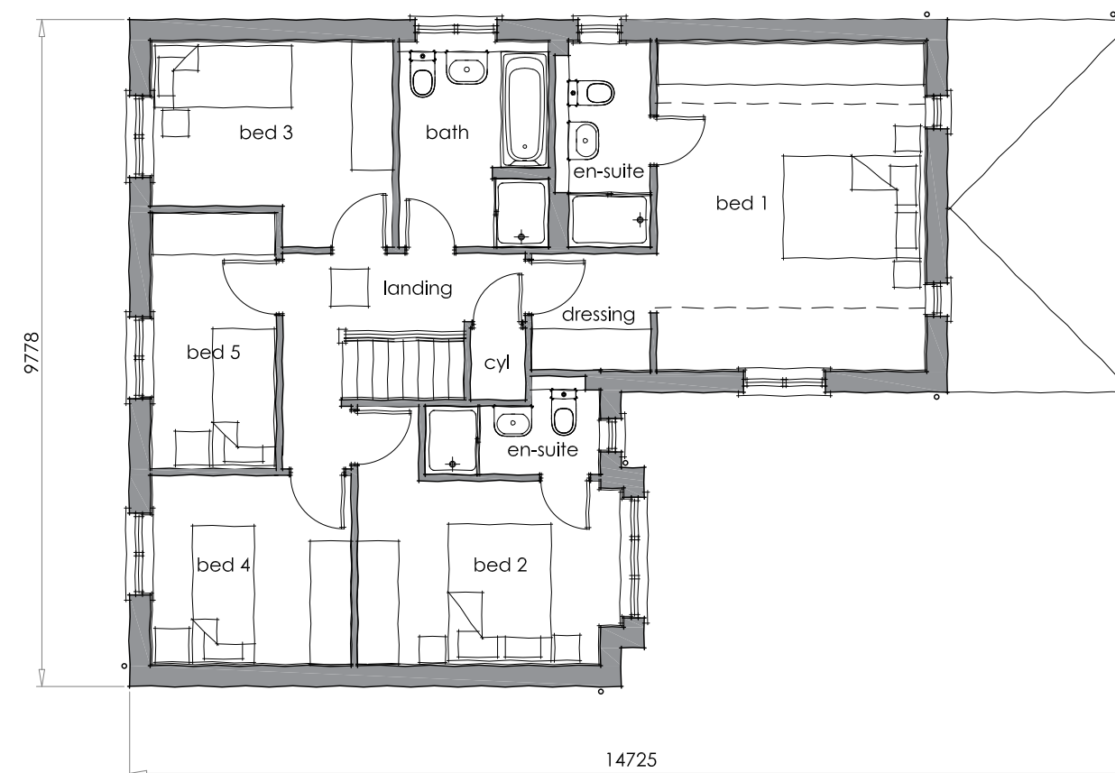
FIRST FLOOR
