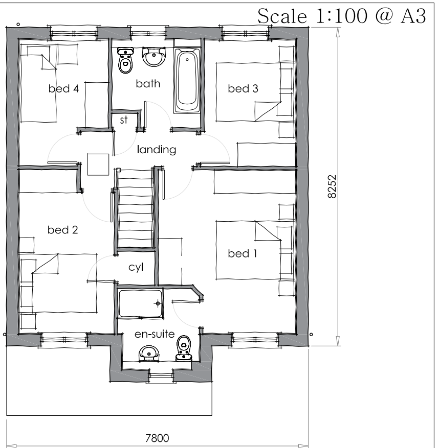
FIRST FLOOR
