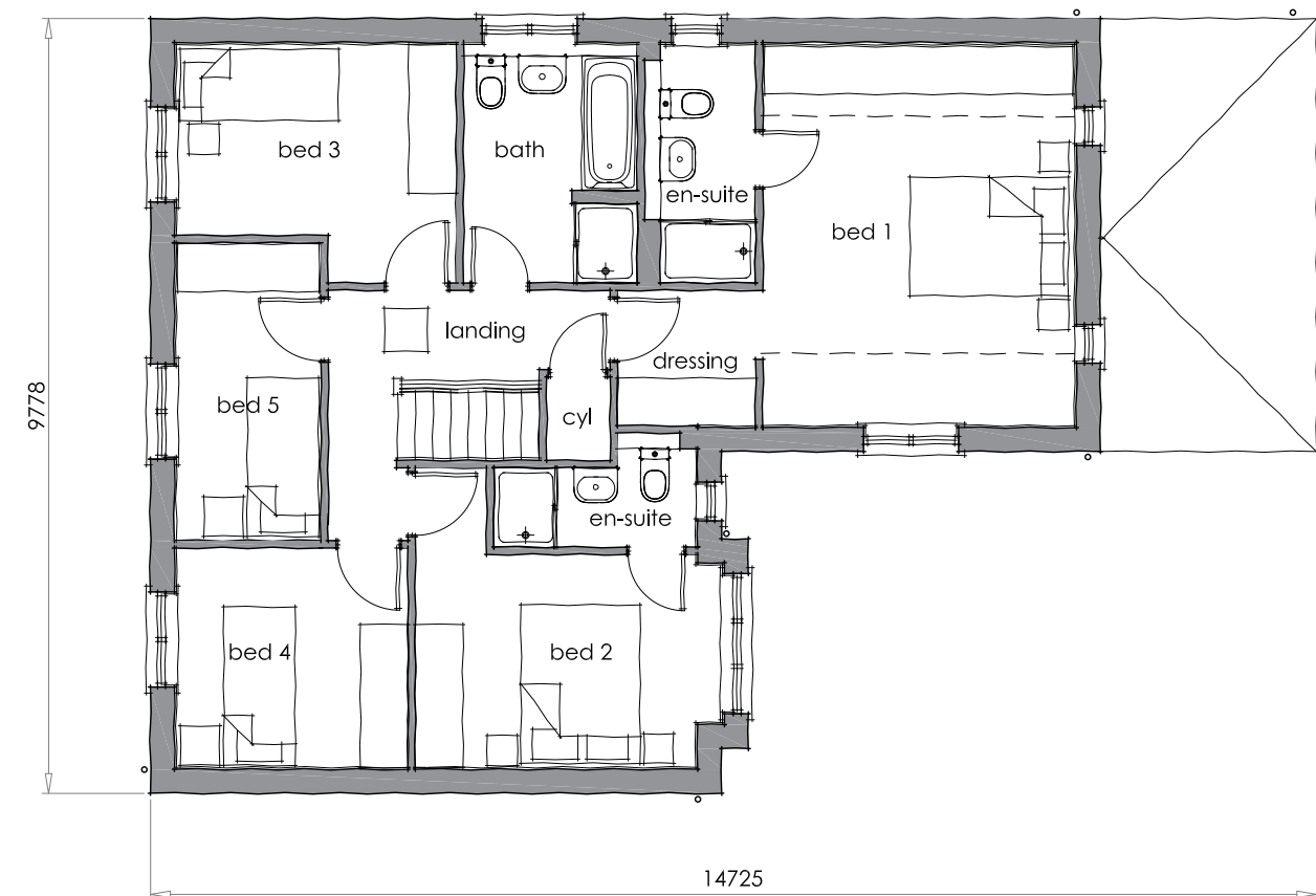
FIRST FLOOR
