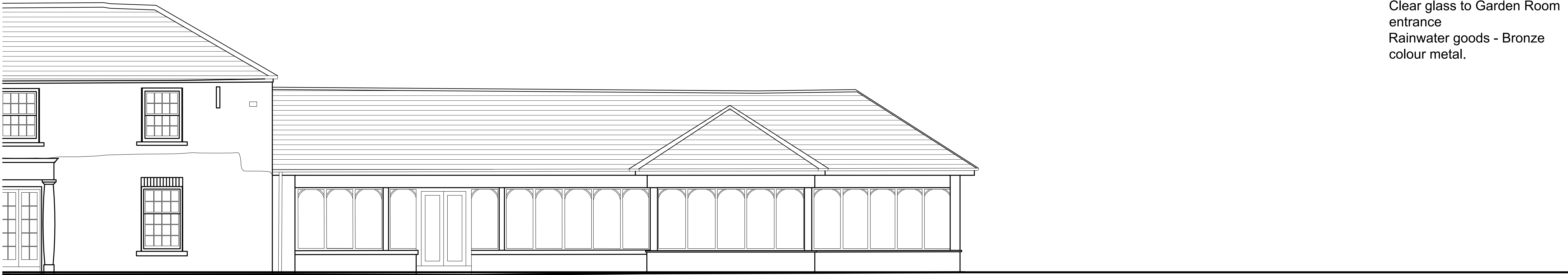
Existing West Elevation
